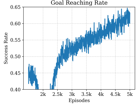
Fig. 4. Goal reaching: progression during Stage 3 training. Initial dip is testament to the fact that the environment is difficult to learn at the start, but the agents progressively get better at reaching goal.
